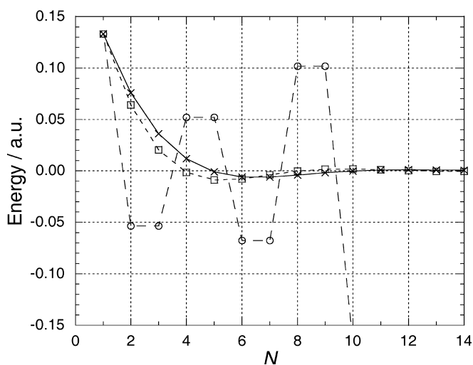
Fig. 7. Same as Fig. 6 but at R = 1.8 Å
