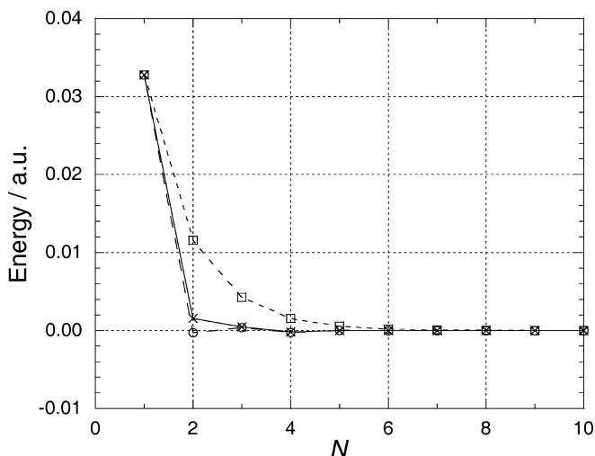
Fig. 10. HF computed using using the MP ( squares ), EN ( circles ), and MAXR c ( crosses ) partitioning methods near the equilibrium geometry ( R = 1.0 Å) upto N = 10 . The energy axis corresponds to (E_N - E_\infty) , where E_N is the N th-order energy and E_\infty is the infinite-order result obtained from the FCI
